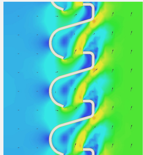
EFD simulation
